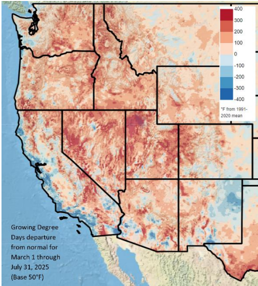
Figure 3 – Western US March through July 2025 growing degree-days (image from Climate Impacts Research Consortium, University of Idaho).
