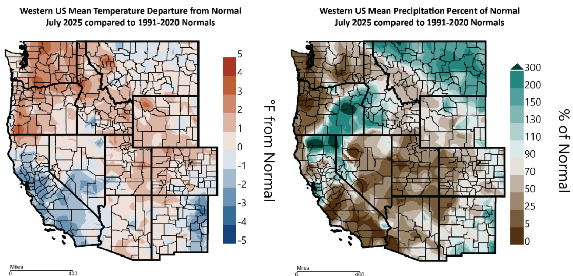
Figure 1 – Western US July 2025 temperature departure from normal (left) and percent of normal precipitation (right; images from Western Regional Climate Center and High Plains Regional Climate Center, 2025)
