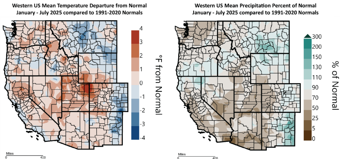
Figure 2 – Western US Year-to-Date (January 1 through July 31, 2025) temperature departure from normal (left) and percent of normal precipitation (right; images from Western Regional Climate Center and High Plains Regional Climate Center, 2025).
